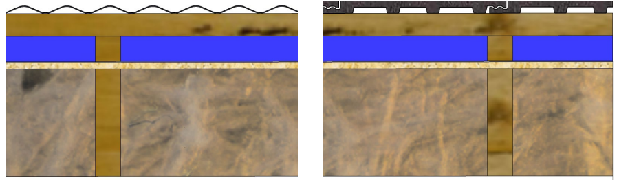
Figure 14: The height of the counter battens can be increased to enhance the airflow and heat removal in summer.
