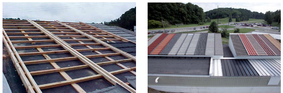
Figure 11: Test roof At Oakridge National Laboratory. (Miller, Wilson & Karagiozis 2006)
