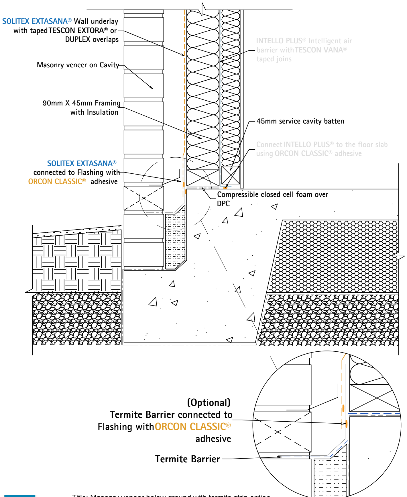
Title: Masonry veneer below ground with termite strip option
